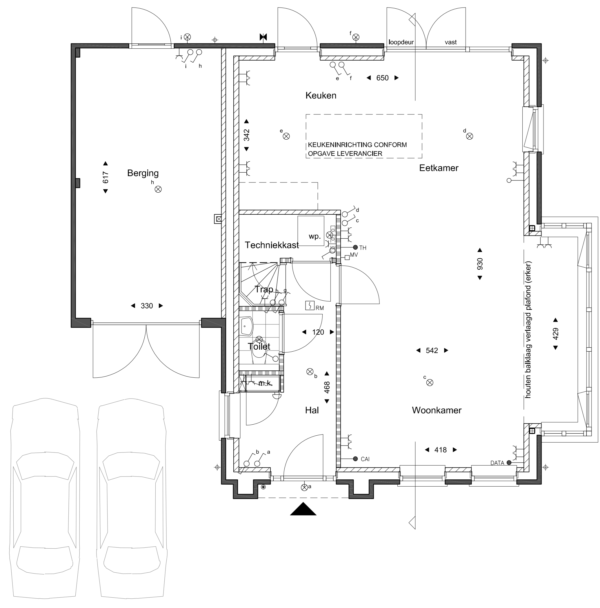
Begane Grond Type A
